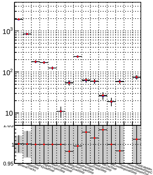
Number 1 DQM_TT__mkFit-DQM_lowptq_mod
