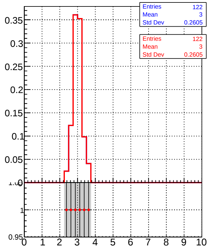
Legend for bottom row plots: DQM_TT_mkFit-DQM_lowptq_orig (grey histogram) DQM_TT_mkFit-DQM_lowptq_mod (red line plot)
