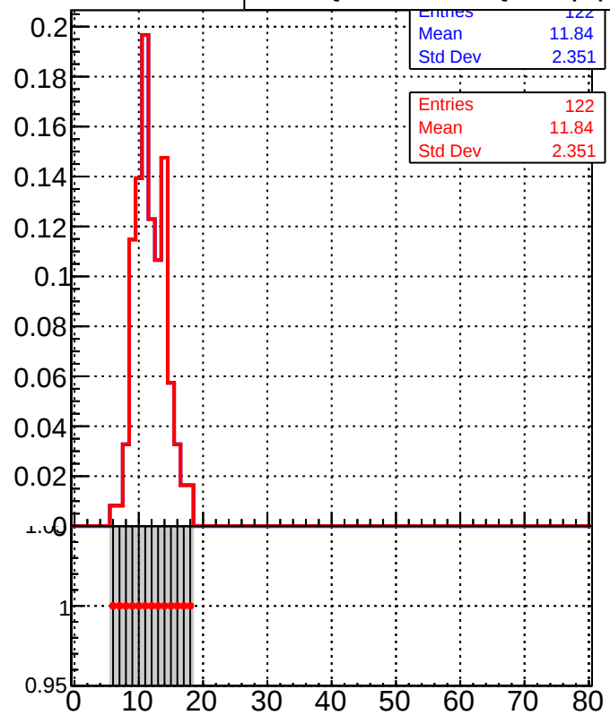
Legend for bottom row plots: DQM_TT_mkFit-DQM_lowptq_orig (grey histogram) DQM_TT_mkFit-DQM_lowptq_mod (red line plot)
