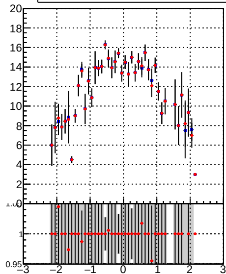
mean hit — DQM_TT_mkFit-DQM_lowptq_orig — DQM_TT_mkFit-DQM_lowptq_mod
