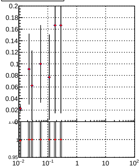
—•— DQM_TT_mkFit-DQM_lowptq_orig —•— DQM_TT_mkFit-DQM_lowptq_mod
