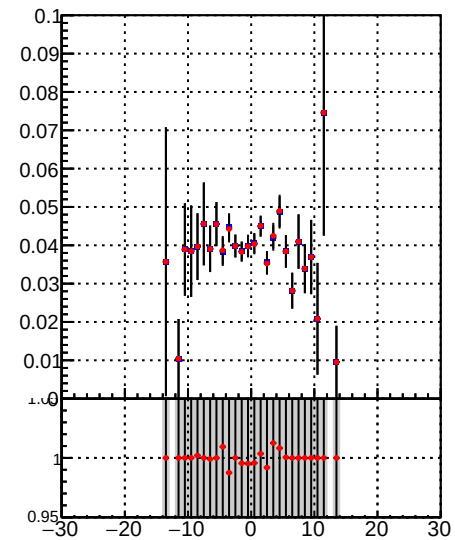
Fake rate vs d —•— DQM TT mkFit-DQM_lowptq_orig —•— DQM TT mkFit-DQM_lowptq_mod
