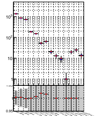
N of reco track vs. \chi^2 DQM_TT mkFit-DQM_lowptq_orig DQM_TT mkFit-DQM_lowptq_mod
