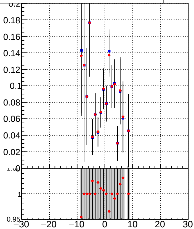
DQM_TT_mkFit-DQM_lowptq_orig DQM_TT_mkFit-DQM_lowptq_mod
