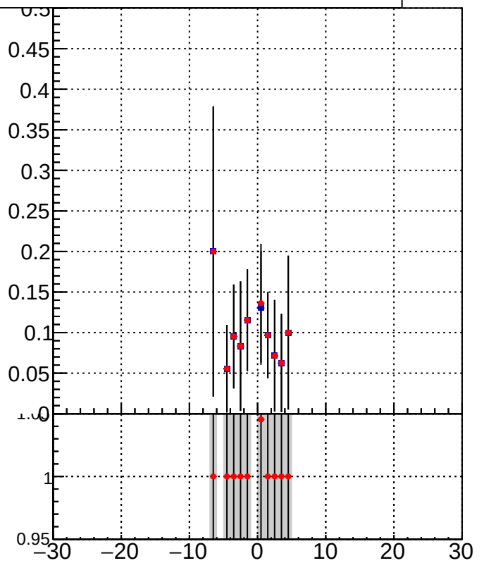
DQM_TT_mkFit-DQM_lowptq_orig DQM_TT_mkFit-DQM_lowptq_mod
