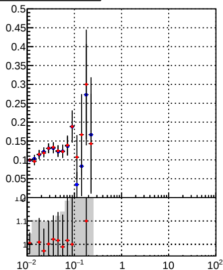
—■— DQM_TT_mkFit-DQM_lowptq_orig —●— DQM_TT_mkFit-DQM_lowptq_mod
