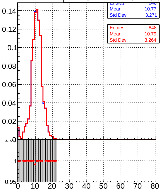
Legend: DQM_TT_mkFit-DQM_lowptq_orig (blue line with squares) DQM_TT_mkFit-DQM_lowptq_mod (red line with circles)
