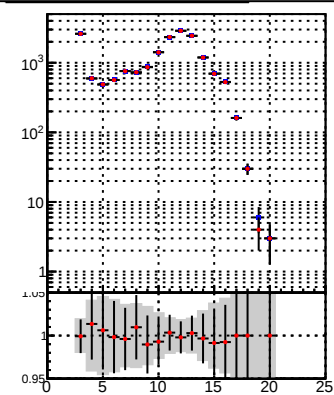
DQM_TT_mkFit-DQM_lowptq_orig DQM_TT_mkFit-DQM_lowptq_mod
