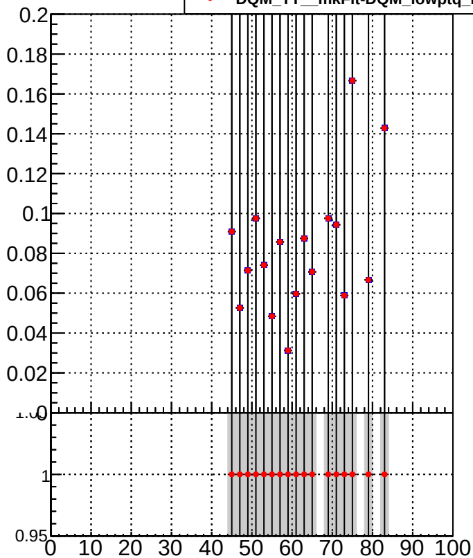
■ DQM_TT_mkFit-DQM_lowptq_orig ● DQM_TT_mkFit-DQM_lowptq_mod
