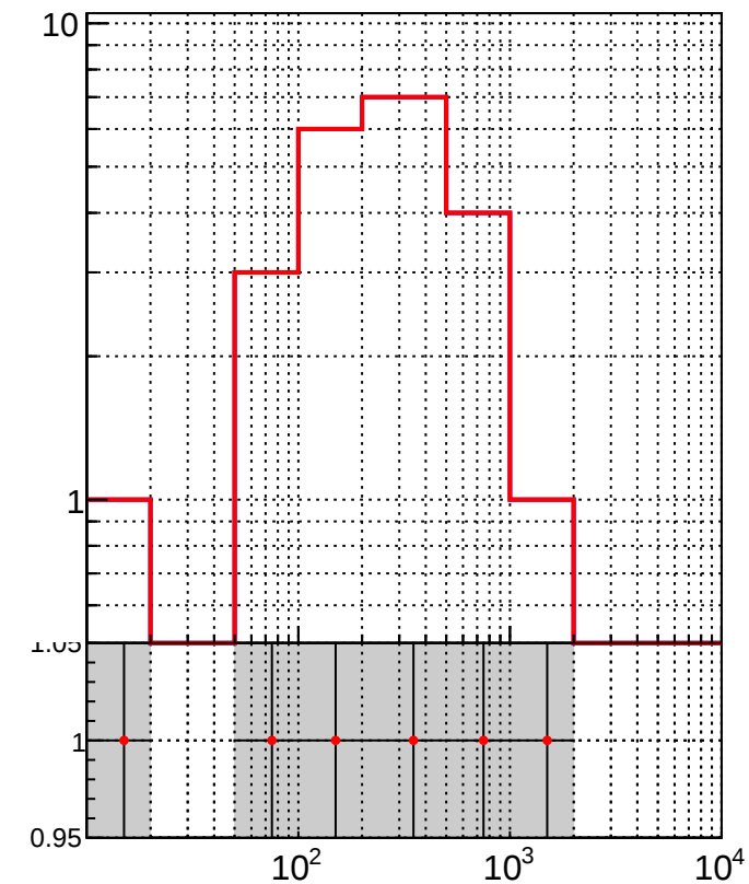
RecoAssoc2GenPVMatchedNotHighest_Pt2
