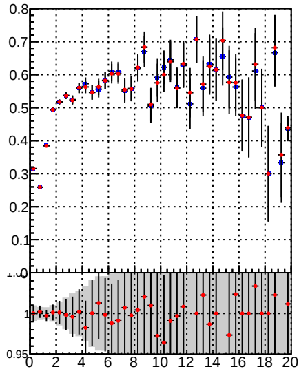
Rate rate vs normalized \chi^2
