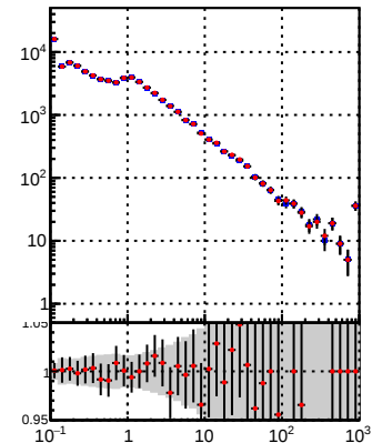
—•— DQM_TT_mkFit-DQM_lowptq_orig —•— DQM_TT_mkFit-DQM_lowptq_mod
