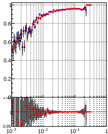
—●— DQM_TT_mkFit-DQM_lowptq_orig —●— DQM_TT_mkFit-DQM_lowptq_mod
