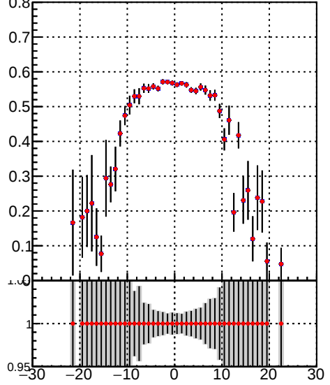
Efficiency vs. sim PV z Legend: DQM_TT_mkFit-DQM_lowptq_orig (blue line) DQM_TT_mkFit-DQM_lowptq_mod (red line)
