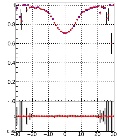
—•— DQM_TT_mkFit-DQM_lowptq_orig —•— DQM_TT_mkFit-DQM_lowptq_mod
