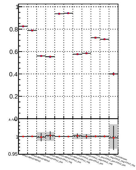
Fake rate vs. — DQM TT mkFit-DQM_lowptq_orig — DQM TT mkFit-DQM_lowptq_mod
