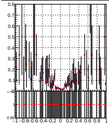
Efficiency vs Dxy(PV) DQM_TT_mkFit-DQM_lowptq_orig DQM_TT_mkFit-DQM_lowptq_mod
