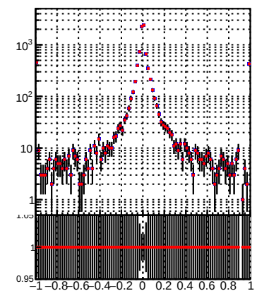
N of sim —●— DQM_TT_mkFit-DQM_lowptq_orig —●— DQM_TT_mkFit-DQM_lowptq_mod
