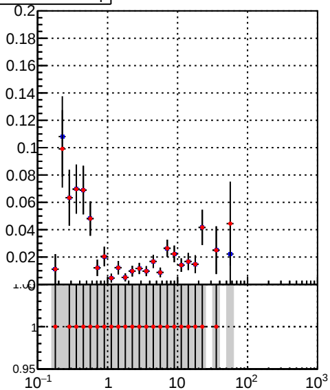
—●— DQM_TT_mkFit-DQM_lowptq_orig —●— DQM_TT_mkFit-DQM_lowptq_mod
