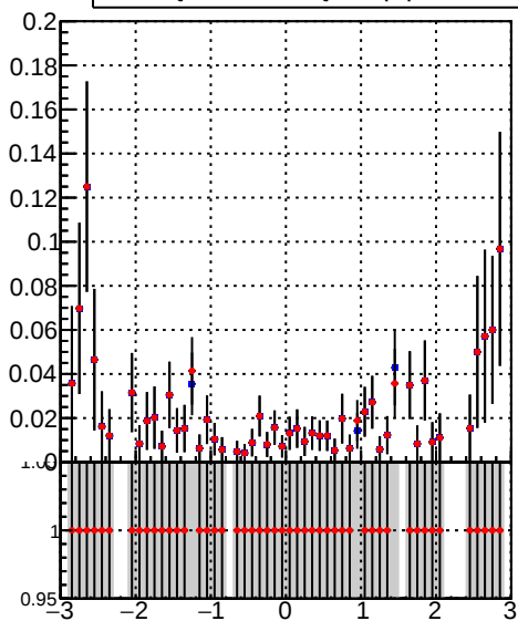
—●— DQM_TT_mkFit-DQM_lowptq_orig —●— DQM_TT_mkFit-DQM_lowptq_mod
