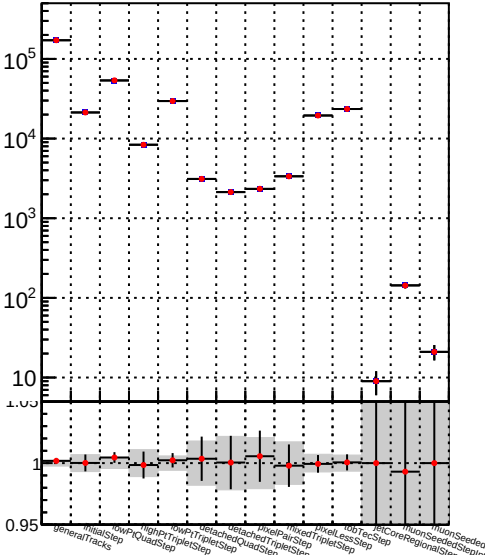
Number 1 DQM_TT_mkFit-DQM_lowptq_mod
