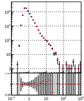
—•— DQM_TT_mkFit-DQM_lowptq_orig —•— DQM_TT_mkFit-DQM_lowptq_mod
