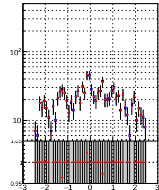
—●— DQM_TT_mkFit-DQM_lowptq_orig —●— DQM_TT_mkFit-DQM_lowptq_mod
