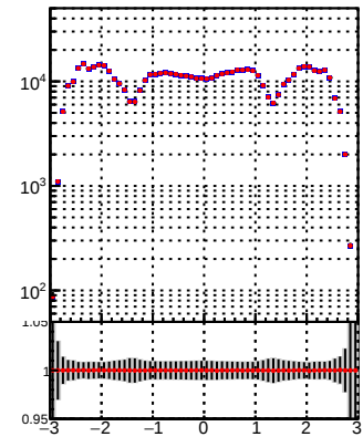
N of reco track vs \eta Legend: DQM_TT_mkFit-DQM_lowptq_orig (blue line with markers) DQM_TT_mkFit-DQM_lowptq_mod (red line with markers)
