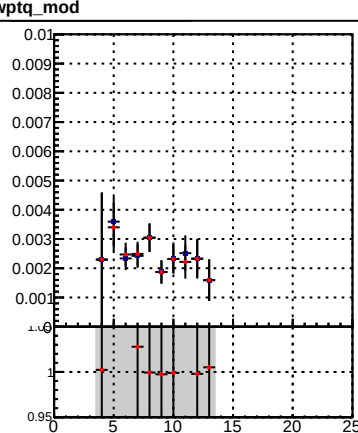
Legend: DQM_TT_mkFit-DQM_lowptq_orig (blue line with dots), DQM_TT_mkFit-DQM_lowptq_mod (red line with dots)
