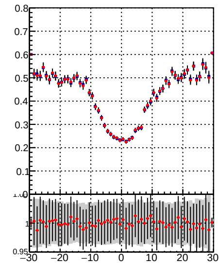
—•— DQM_TT_mkFit-DQM_lowptq_orig —•— DQM_TT_mkFit-DQM_lowptq_mod
