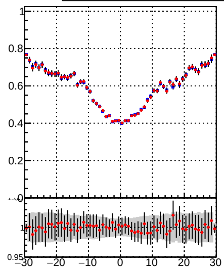
—•— DQM_TT_mkFit-DQM_lowptq_orig —•— DQM_TT_mkFit-DQM_lowptq_mod
