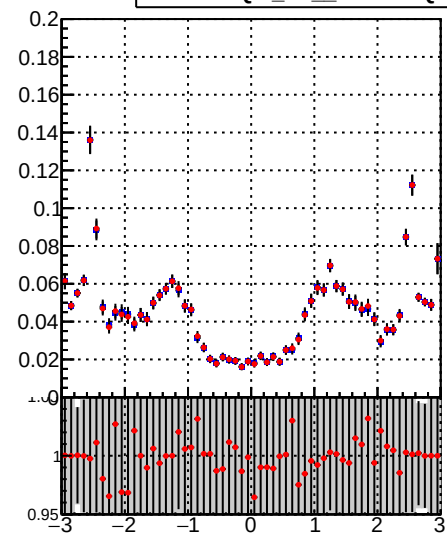
—•— DQM_TT_mkFit-DQM_lowptq_orig —•— DQM_TT_mkFit-DQM_lowptq_mod
