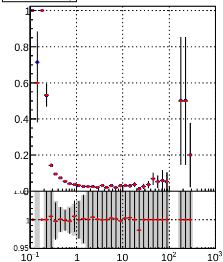
—•— DQM_TT_mkFit-DQM_lowptq_orig —•— DQM_TT_mkFit-DQM_lowptq_mod
