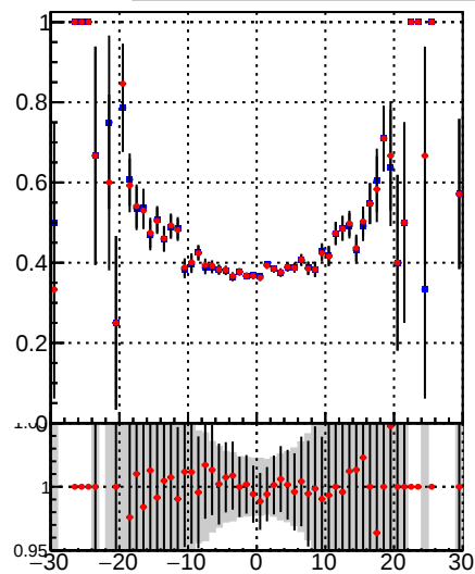
—•— DQM_TT_mkFit-DQM_lowptq_orig —•— DQM_TT_mkFit-DQM_lowptq_mod
