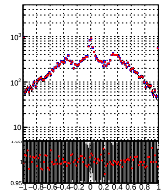
█ DQM_TT_mkFit-DQM_lowptq_orig █ DQM_TT_mkFit-DQM_lowptq_mod
