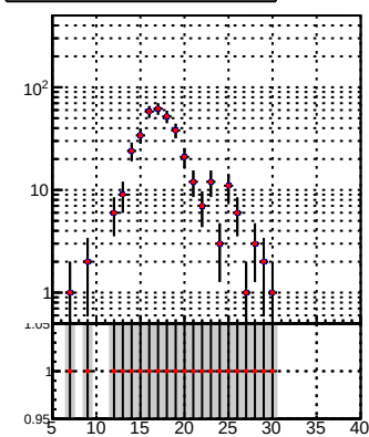
—•— DQM_TT_mkFit-DQM_lowptq_orig —•— DQM_TT_mkFit-DQM_lowptq_mod
