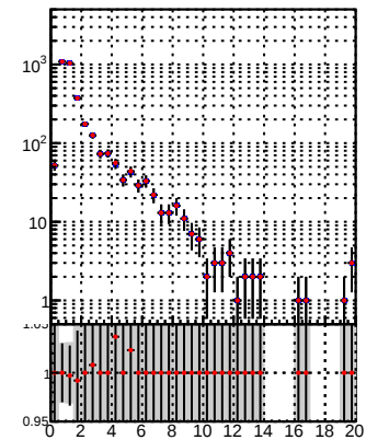
N of reco track vs. —●— DQM TT mkFit-DQM_lowptq_orig —●— DQM TT mkFit-DQM_lowptq_mod
