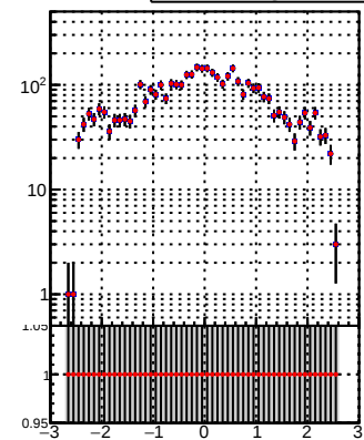
—•— DQM_TT_mkFit-DQM_lowptq_orig —•— DQM_TT_mkFit-DQM_lowptq_mod
