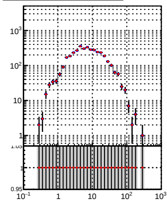
—•— DQM_TT_mkFit-DQM_lowptq_orig —•— DQM_TT_mkFit-DQM_lowptq_mod
