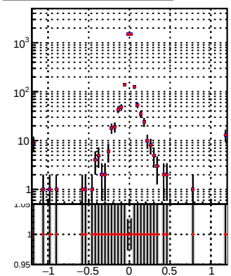
N of associated (recoToSim) tracks vs dz(PV)
