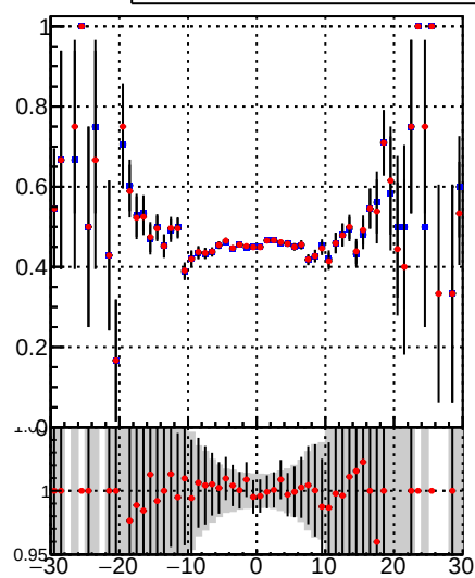
■ DQM_TT_mkFit-DQM_lowptq_orig ● DQM_TT_mkFit-DQM_lowptq_mod
