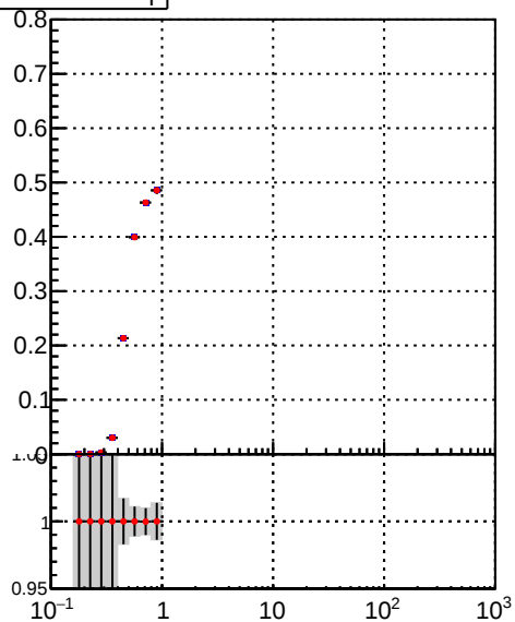
DQM_TT_mkFit-DQM_lowptq_orig DQM_TT_mkFit-DQM_lowptq_modi3
