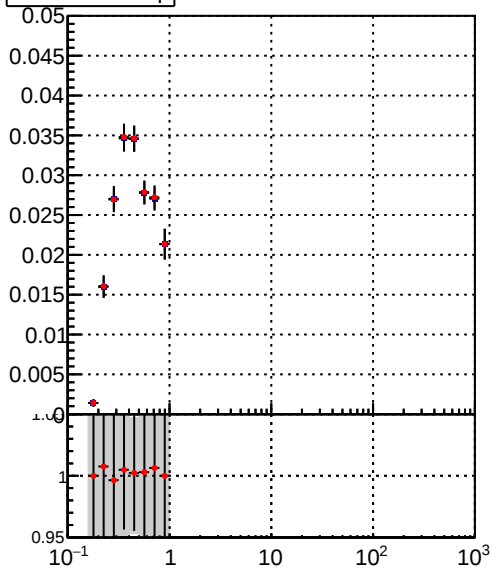
Legend: — DQM_TT_mkFit-DQM_lowptq_orig — DQM_TT_mkFit-DQM_lowptq_modi3
