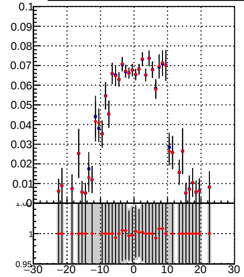
Efficiency vs vertpos Legend: DQM_TT_mkFit-DQM_lowptq_orig DQM_TT_mkFit-DQM_lowptq_modi3
