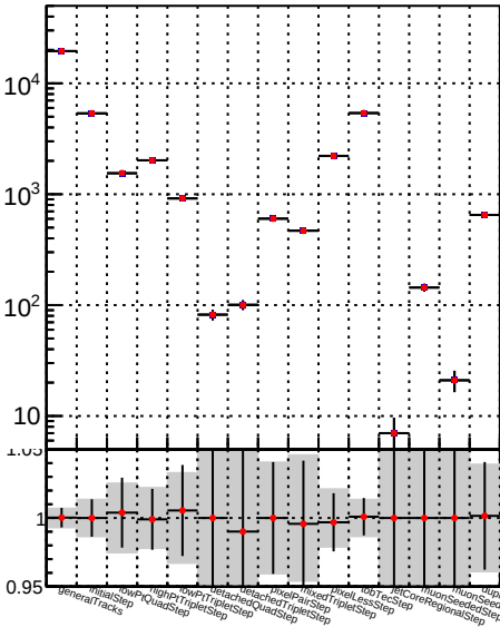
Number —●— DQM_TT_mkFit-DQM_lowptq_modi3
