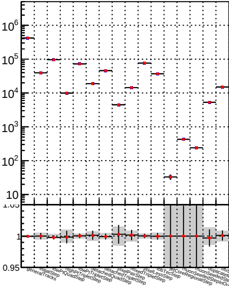
Number —●— DQM_TT_mkFit-DQM_lowptq_mc
