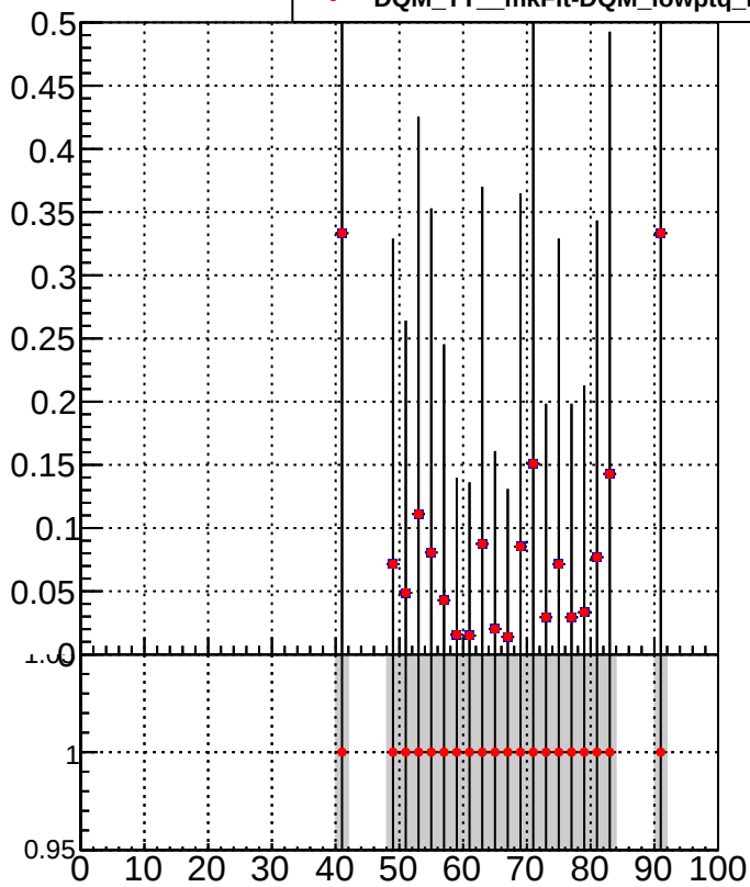
■ DQM_TT_mkFit-DQM_lowptq_orig ● DQM_TT_mkFit-DQM_lowptq_modi3
