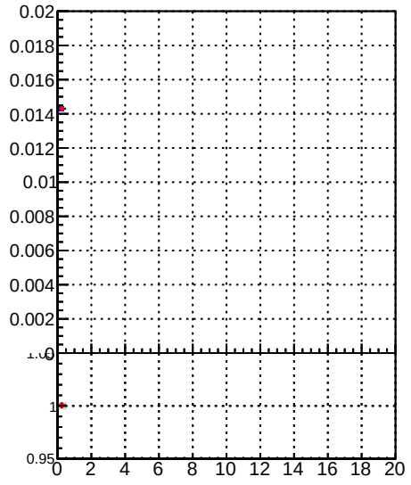
Fake rate vs. — DQM TT mkFit-DQM_lowptq_orig — DQM TT mkFit-DQM_lowptq_modi3
