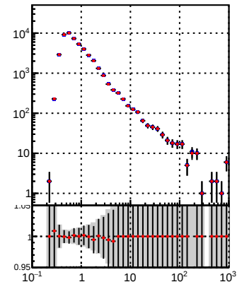
—●— DQM_TT_mkFit-DQM_lowptq_orig —●— DQM_TT_mkFit-DQM_lowptq_modi3
