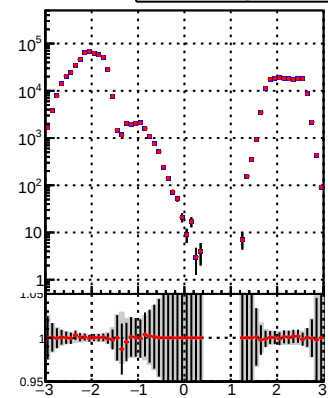
—●— DQM_TT_mkFit-DQM_lowptq_orig —●— DQM_TT_mkFit-DQM_lowptq_modi3
