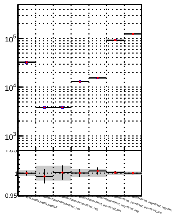
N of reco track vs. \chi^2 —•— DQM TT mkFit-DQM_lowptq_orig —•— DQM TT mkFit-DQM_lowptq_modi3
