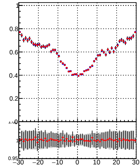
—●— DQM_TT_mkFit-DQM_lowptq_orig —●— DQM_TT_mkFit-DQM_lowptq_modi3
