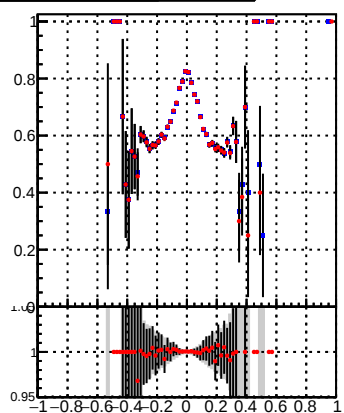
DQM_TT_mkFit-DQM_lowptq_modi3
