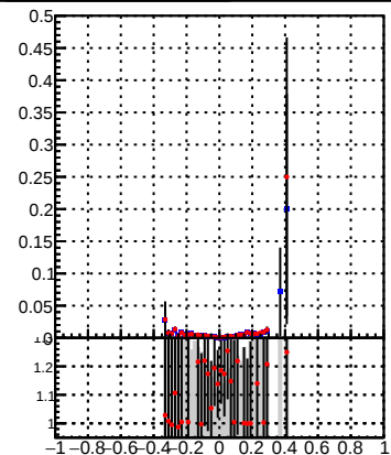
DQM_TT_mkFit-DQM_lowptq_orig
