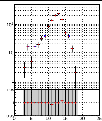
—•— DQM_TT_mkFit-DQM_lowptq_orig —•— DQM_TT_mkFit-DQM_lowptq_modi3
