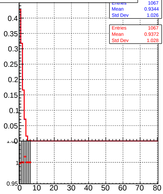
Legend for bottom row plots: DQM_TT_mkFit-DQM_lowptq_orig (Blue line with squares) DQM_TT_mkFit-DQM_lowptq_modi3 (Red line with circles)
