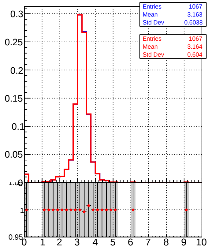
Legend for bottom row plots: DQM_TT_mkFit-DQM_lowptq_orig (Blue line with squares) DQM_TT_mkFit-DQM_lowptq_modi3 (Red line with circles)
